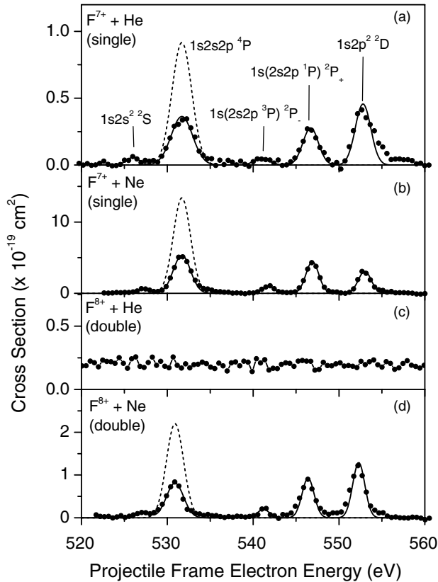
FIG. 1. Measured spectra for single electron transfer to F^{7+} and double electron transfer to F^{8+} for 1.1 MeV/u collisions of these ions with He and Ne. The observed 1s2l2l' intermediate states are indicated (for F^{8+} + \text{He} no measurable intensity was observed for these states). The dashed curves represent the true intensity of the 1s2s2p^4P state after correction for instrumental effects due to the long lifetime of this state (see text).
