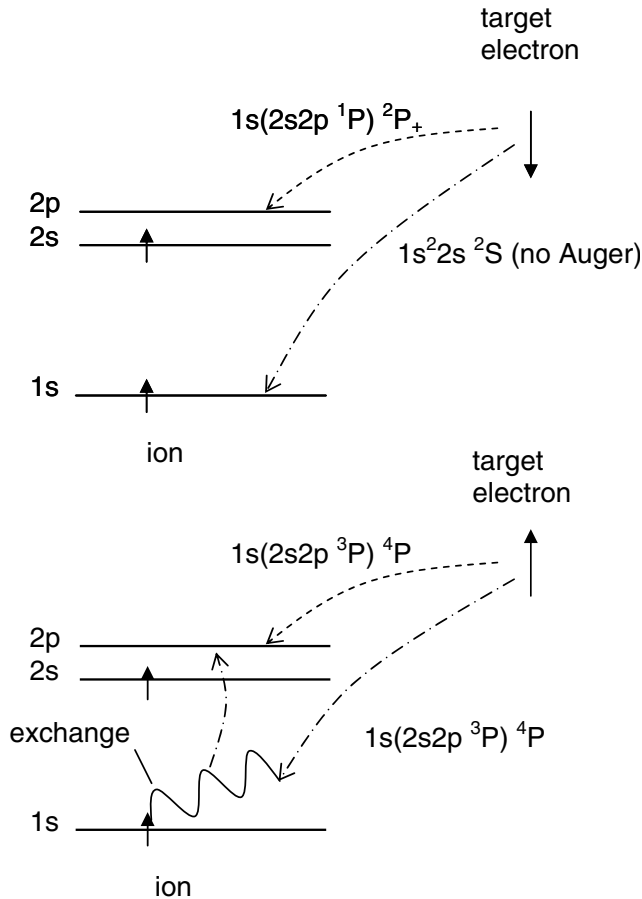
FIG. 2. Pathways for formation of the 1s(2s2p^1P)^2P_+ and 1s(2s2p^3P)^4P states by transfer of a target electron antialigned (upper part) and aligned (lower part), respectively, with the F^{7+}(1s2s^3S) projectile electrons. The Pauli exchange interaction contributing to formation of the 1s2s2p^4P state is indicated by the wavy line connecting the 1s electron and the incoming target electron.
