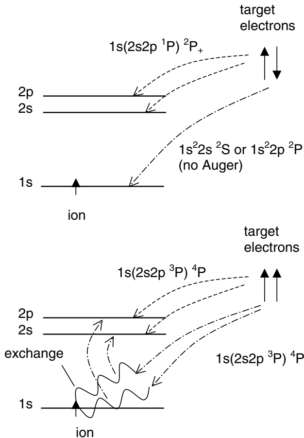
FIG. 3. Pathways for formation of the 1s(2s2p^1P)^2P_+ and 1s(2s2p^3P)^4P states by transfer of target electrons with one spin aligned and one spin antialigned (upper part) and both spins aligned (lower part), respectively, with the F^{8+}(1s) projectile electron. The double Pauli exchange interaction contributing to formation of the 1s2s2p^4P state is indicated by the wavy lines connecting the 1s electron with the incoming target electrons.
