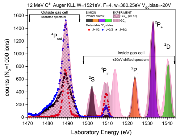
Figure 1. Comparison of SIMION simulations to experimental spectra. In both cases, the ^4P line is seen to be broken into two separate components, the unshifted line from electrons emitted outside the gas cell and the shifted line from electrons produced from inside the gas cell which is biased at V_{GC} = -20V . SIMION results (scaled to the experimental spectrum) are seen to nicely reproduce the line shapes of both the metastable ^4P state and the prompt doublet states.
